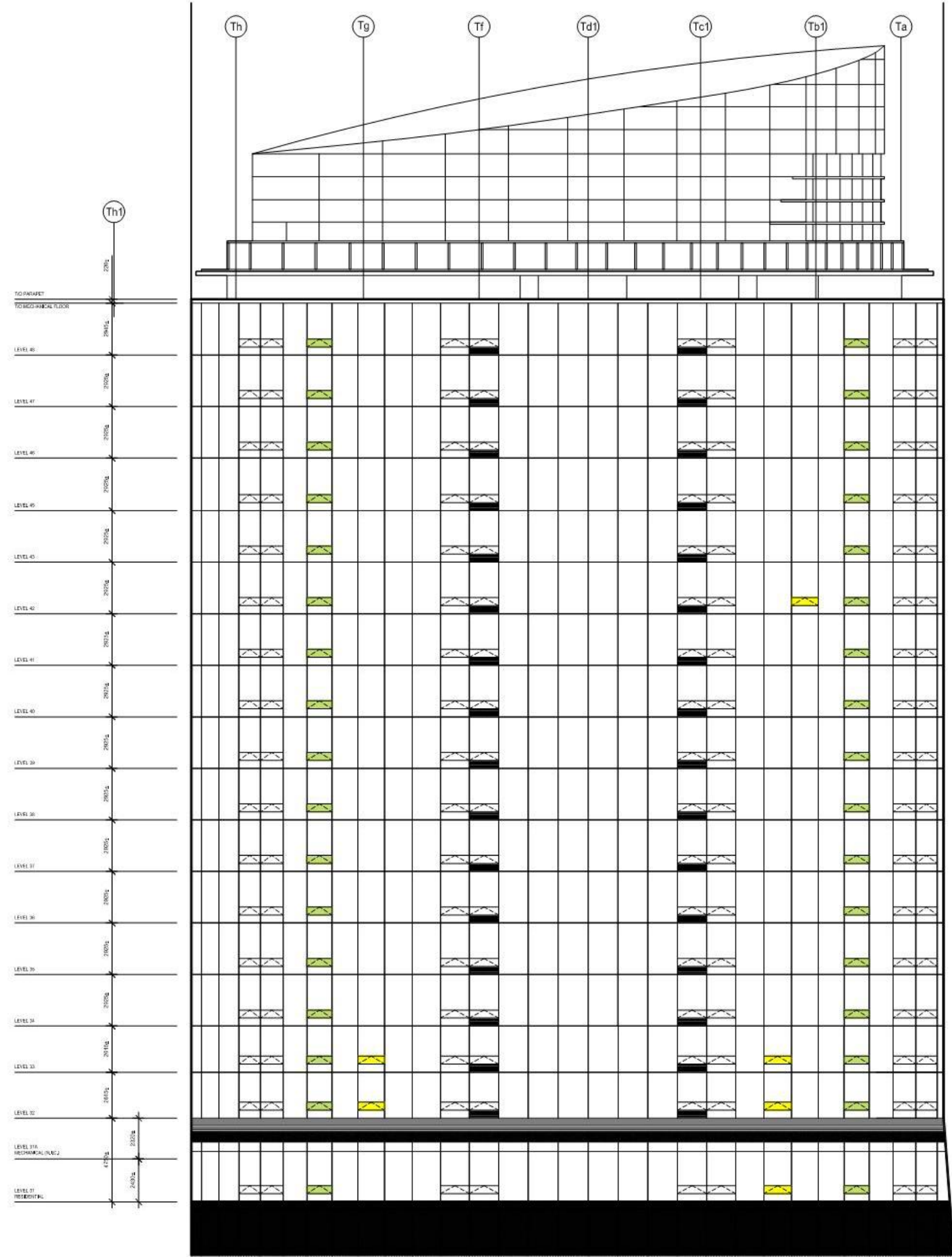
PARTIAL NORTH ELEVATION FOR WINDOW TYPE TAGS REFER TO A-3.02
